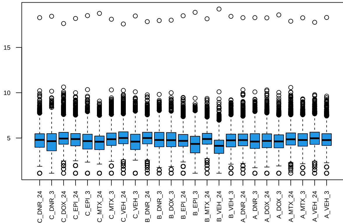
Boxplot of \text{Log}_2 counts-per-million
